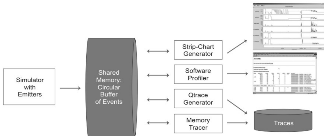
Figure 47. Emitter architecture
